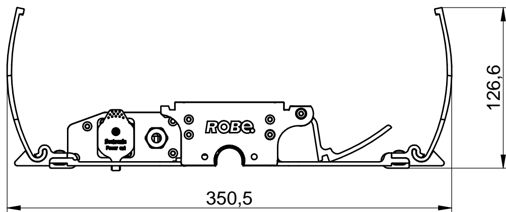
ALTERNATE VIEW Top covers in open position
