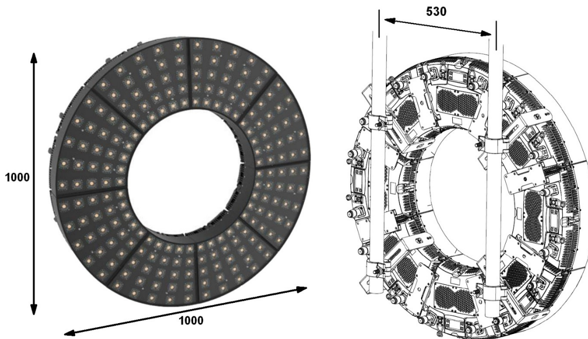
Figure 16. KNV Arc circular array dimensions
