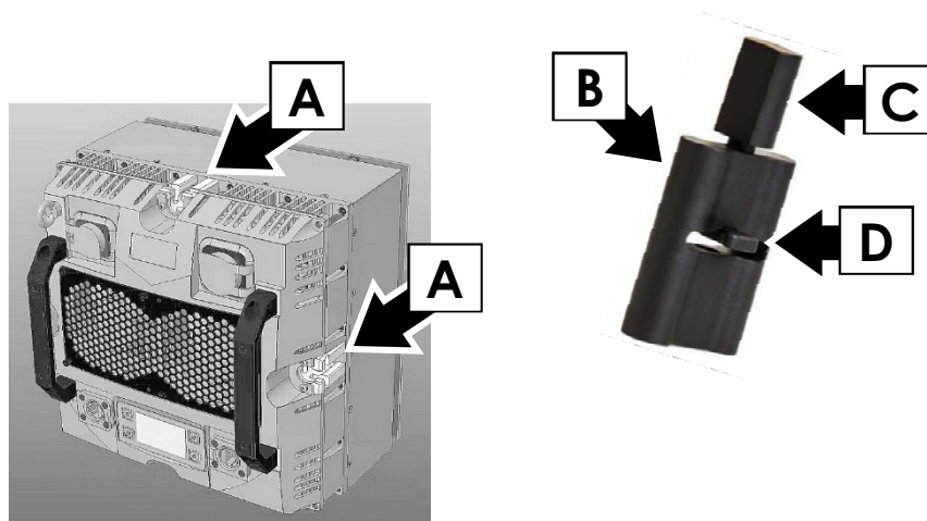
Figure 6. Using a KNV Fixture Connector
